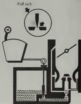
FIGURE 3-11. Needle-type mixture control system.
